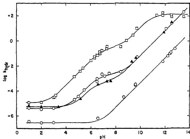
Figure 1. Plots of \log k_{\text{hydr}} ( k_{\text{hydr}} in units of \text{sec}^{-1} ) vs. pH for the hydrolysis of esters: I ( \square ), III ( \circ ), IV ( \blacktriangle ), and V ( \circ ). The points are experimental and the lines calculated from eq 3 for I, eq 4 for III and IV, and eq 5 for V. Between steady-state and preequilibrium conditions reaction 9 predicts an A \rightleftharpoons B \rightarrow C process for which a lag phase should exist in the production of C. Due to the magnitude of the rate constant for o -nitrophenolate release at this pH differentiation of a lag phase from mixing time on the stopped-flow spectrophotometer could not be made. With the exception of the small pH range around 11, (9) predicts pseudo-first-order kinetics. In Figure 1 the values of \log k_{\text{obsd}} pertain to these pseudo-first-order rate constants.
