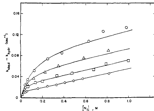
Figure 3. Plots of k_{\text{obsd}} - k_{\text{hydr}} vs. the concentration of nucleophile in its free base form for the hydrolysis of ester III: top, morpholine ( \circ , pH 8.66; \Delta , pH 8.47; \square , pH 8.28); middle, Tris ( \circ , pH 8.30; \Delta , pH 8.13; \square , pH 7.85); bottom, N-ethylmorpholine ( \circ , pH 8.43; \Delta , pH 8.23; \square , pH 8.02; \circ , pH 7.78). The points are experimental and the lines theoretical having been derived from eq 20 using the constants of Table V.
